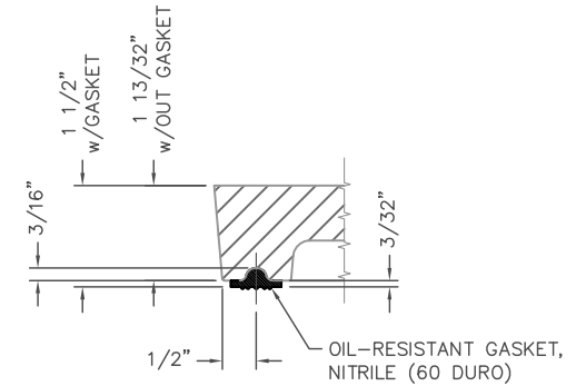
"T SEAL" GASKET DETAIL SCALE 1:2
